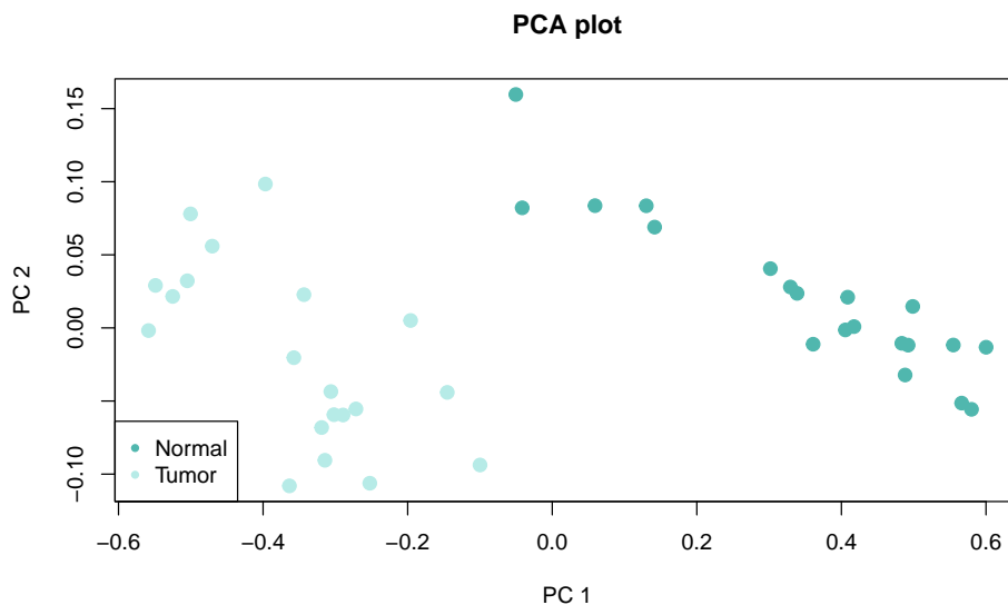
Figure 12: PCA plot
